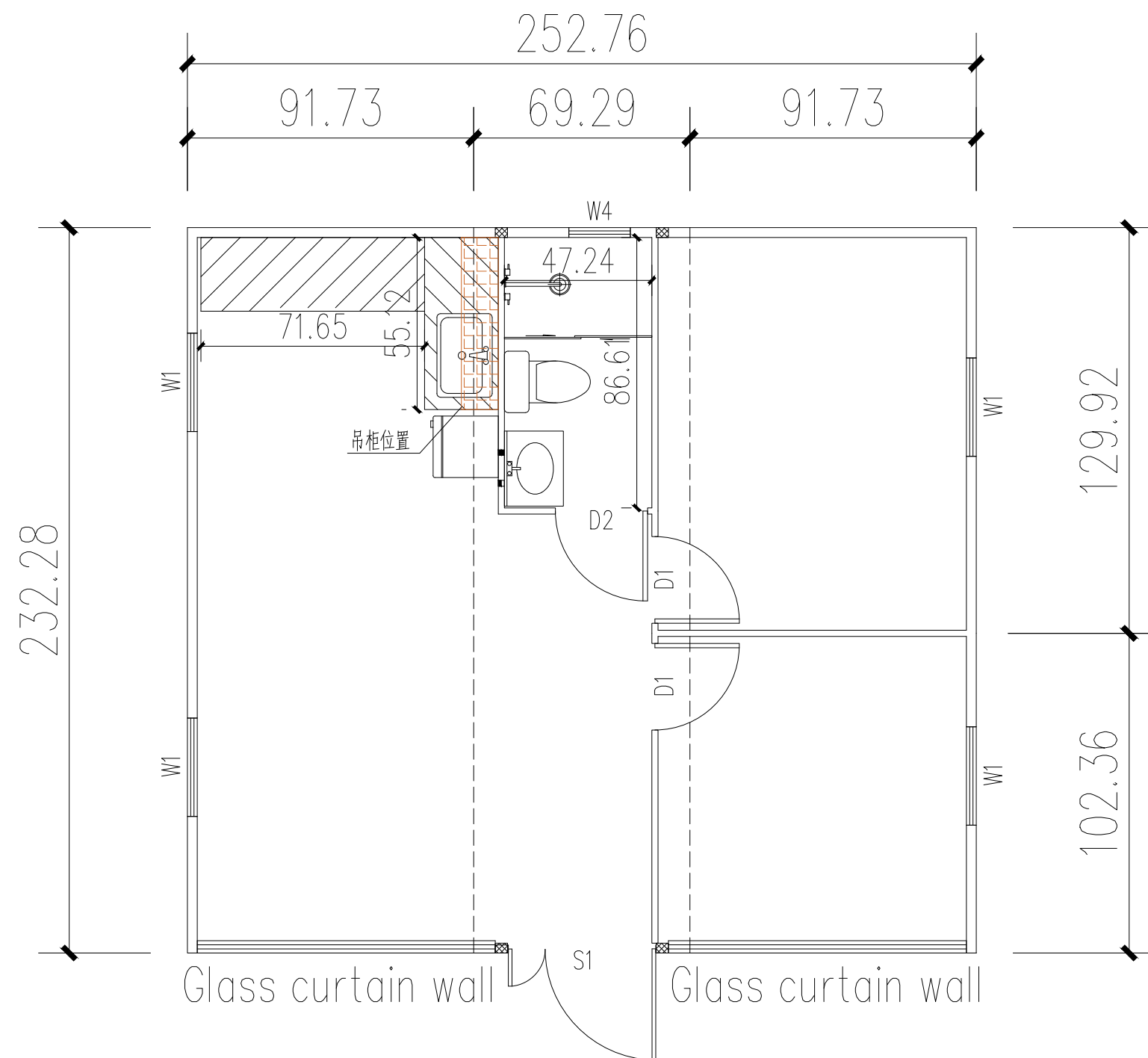
20' double wing plan
