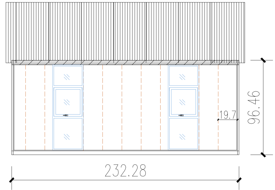
Left elevation
