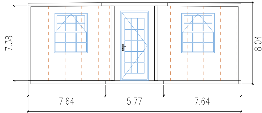
21.06 Front elevation view
