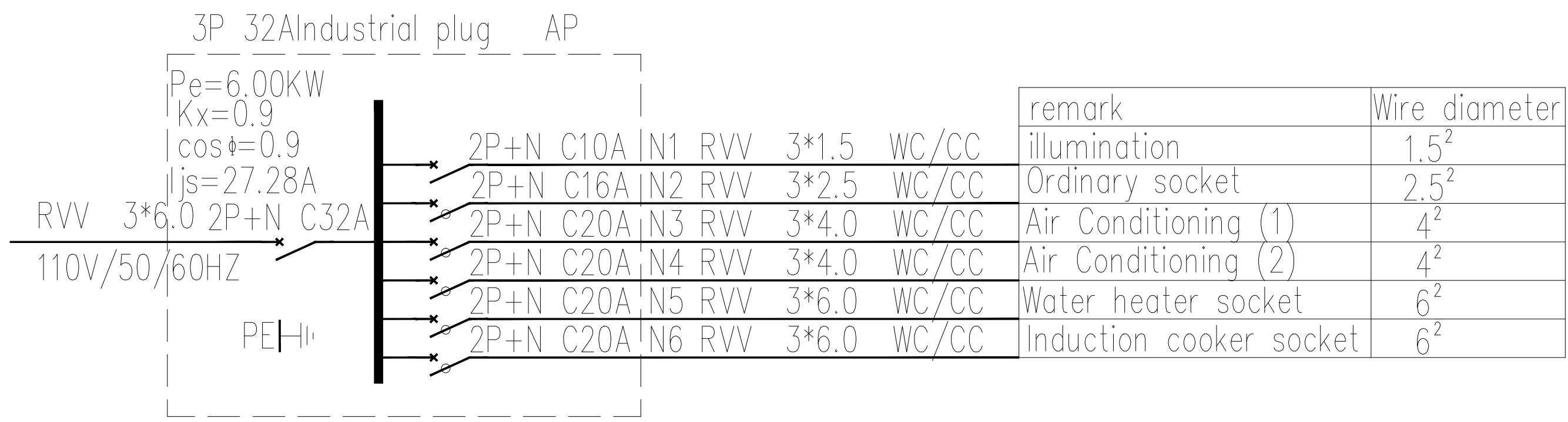
American standard certified electrical system diagram
