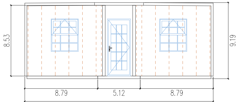
22.7 Front elevation view
