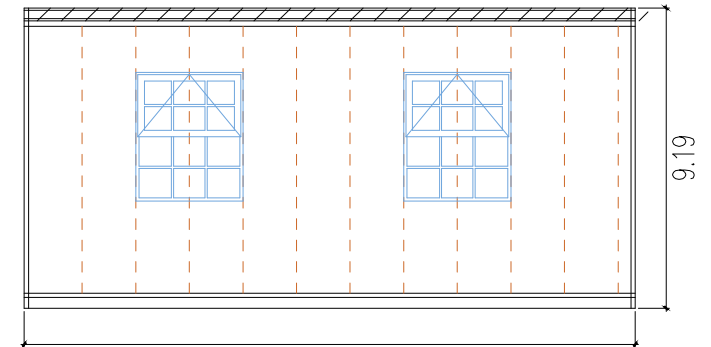
18.7 Right elevation view
