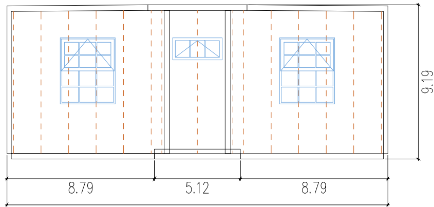
22.7 Rear elevation view
