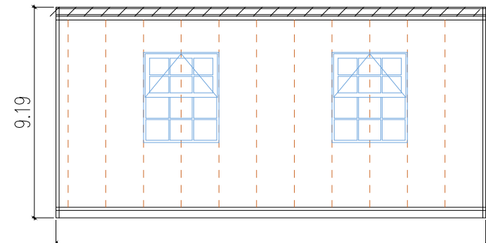
18.7 Left elevation view
