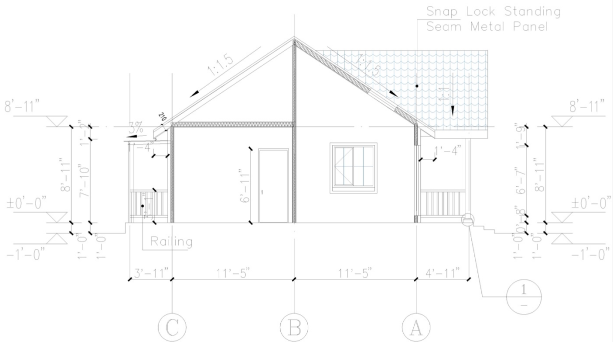
①-① sectional view 1:100
