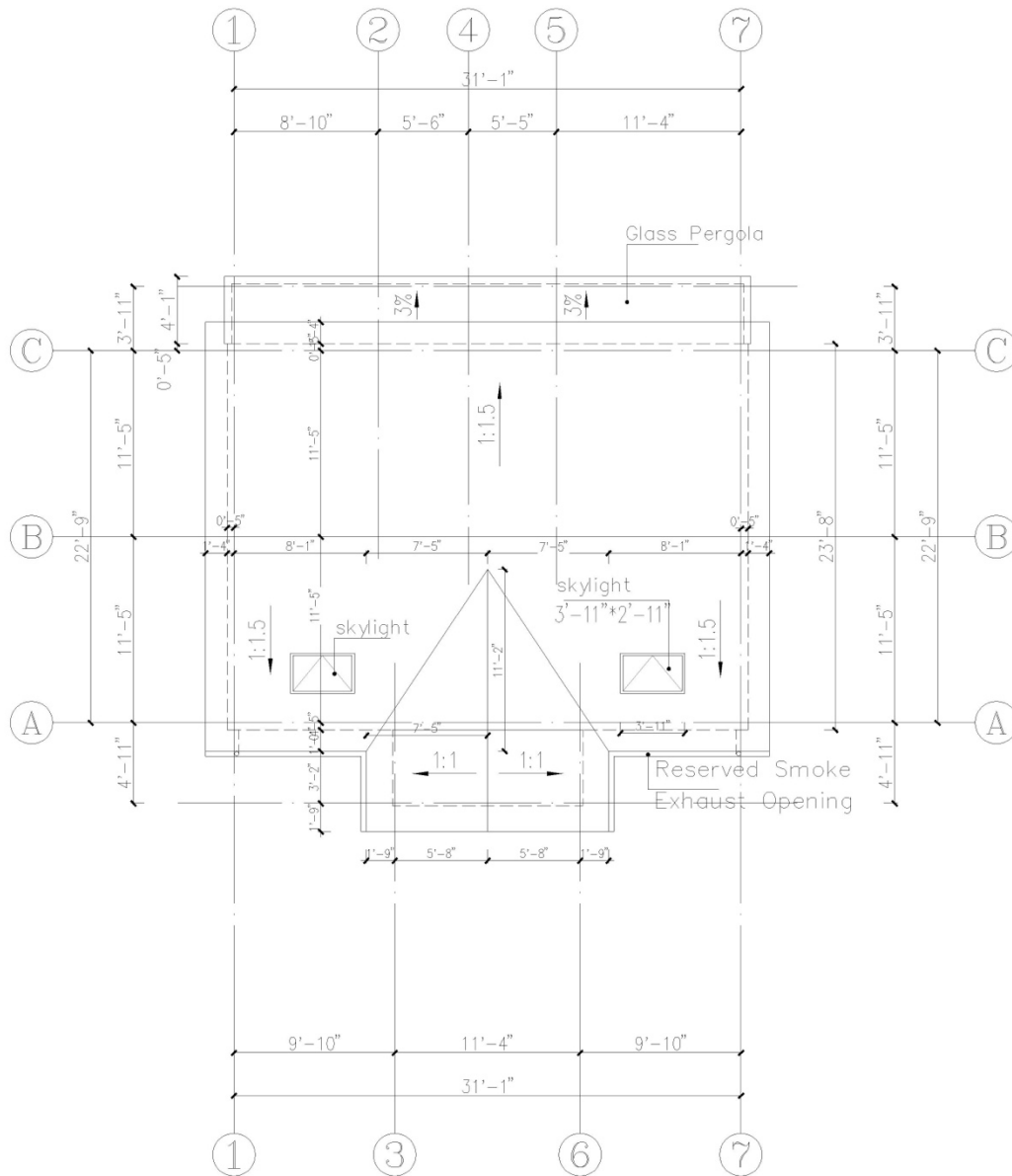
Roof plan 1:100
