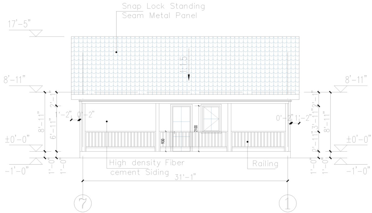
⑦-① Axial Elevation Drawing 1:100
