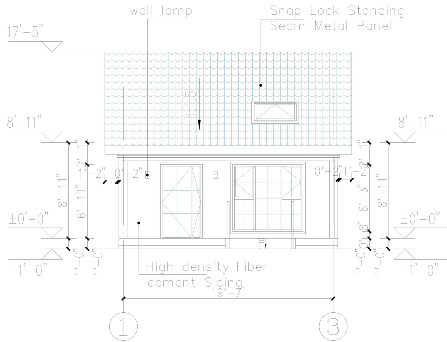
①-③Axial Elevation Drawing 1:100
