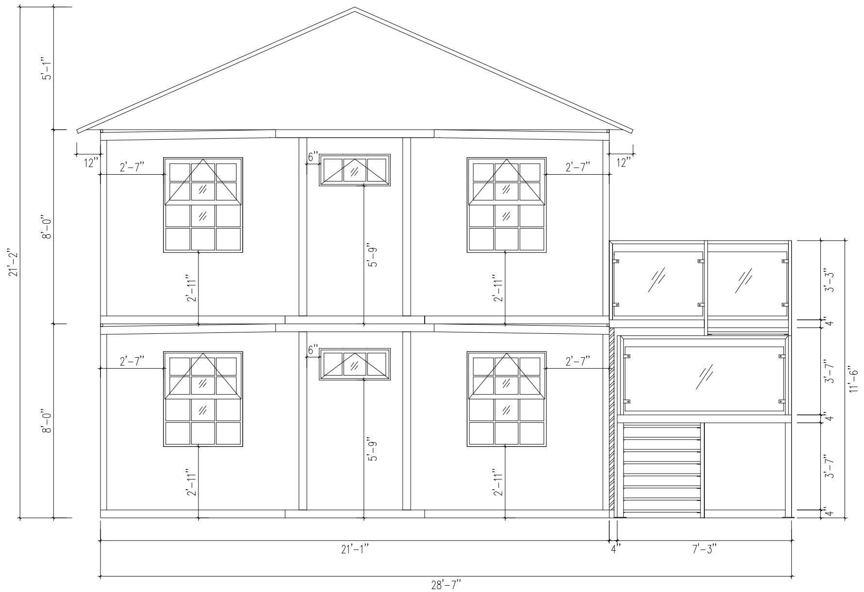
Rear elevation view
