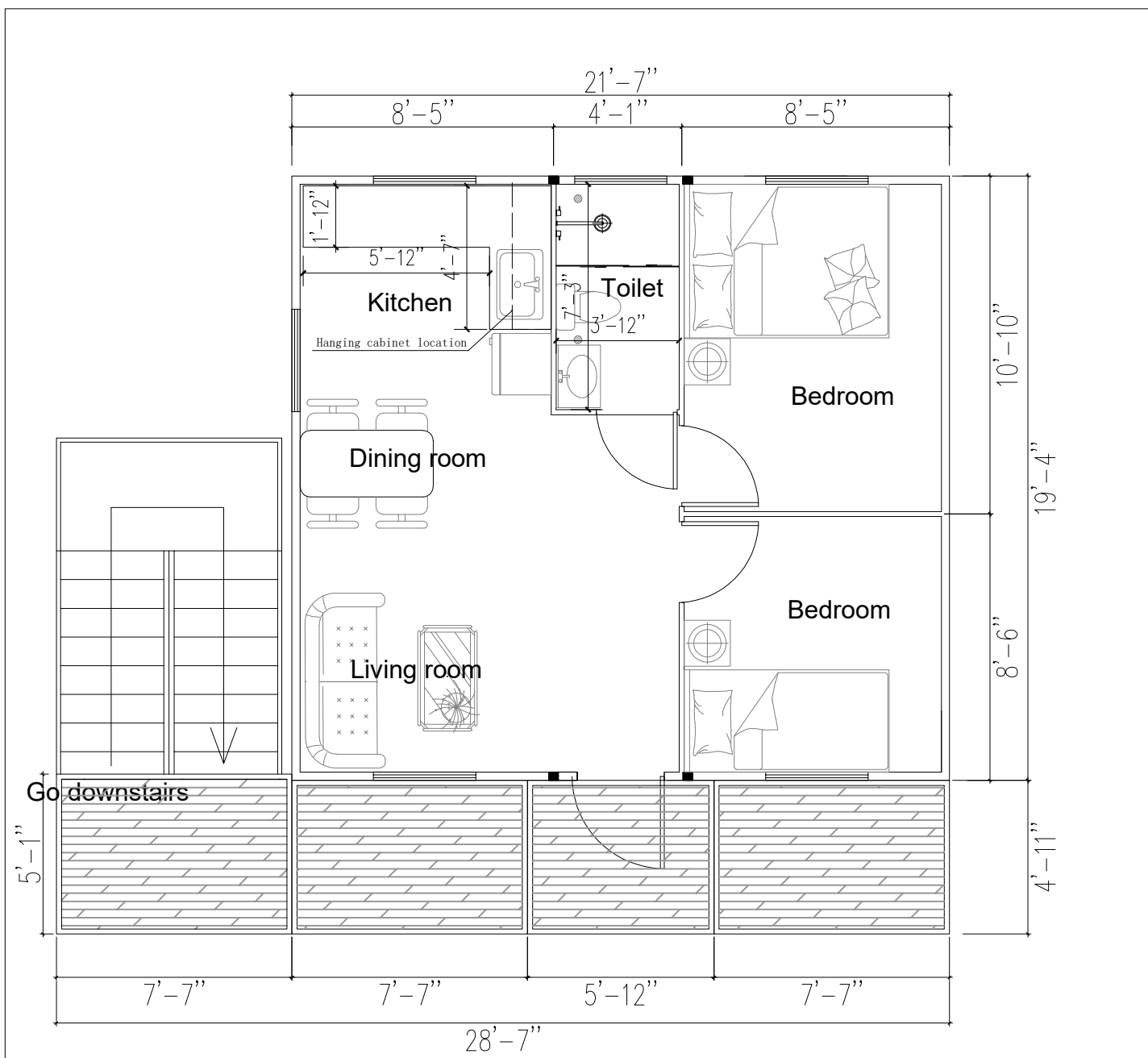
Second floor layout plan
